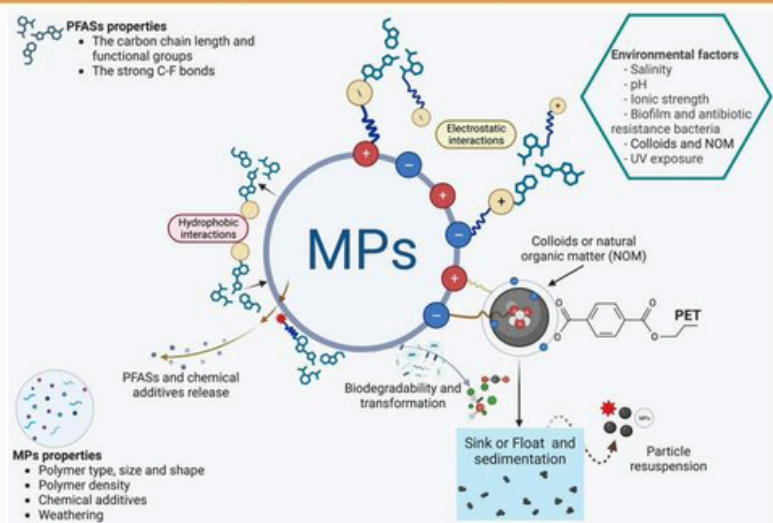
Figure 1. Mechanism of microplastic-promoted PFASs in environmental interaction (adapted from ref 17). Created with BioRender.com.
